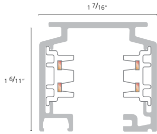
2-Circuit Track
