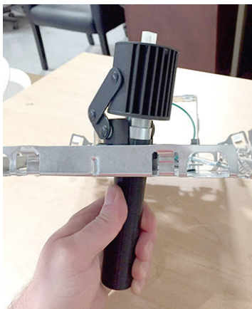
3 - Use the threaded side of the adjustment tool to aim/ focus the light.
