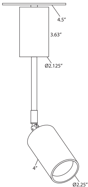
Canopy Plate with Stem
