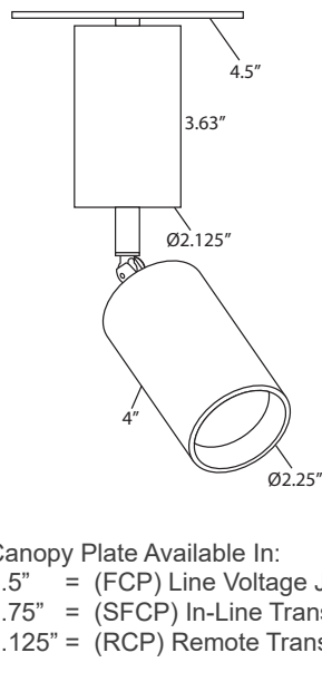
Flat Canopy Plate
