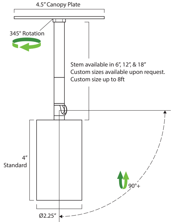
Trimless - Wood
