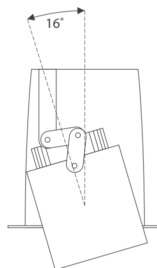
Wall Wash Down Light
