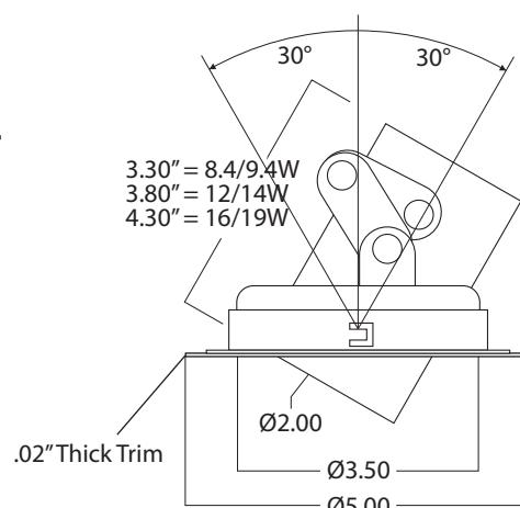
Semi-Recessed
