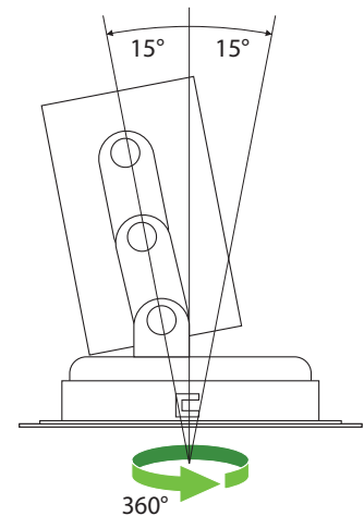
100% Recessed
